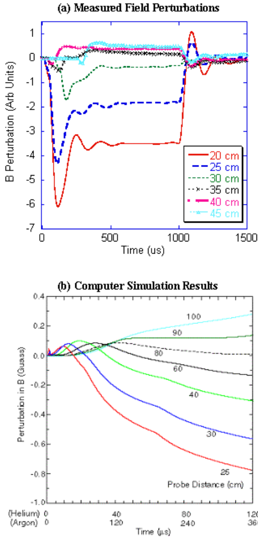
Figure 1. An example a single column figure showing a comparison of (a) the observed magnetic field perturbations and (b) computer simulations. Caption should be Font Size 11, left/right justified, and aligned with the column.
